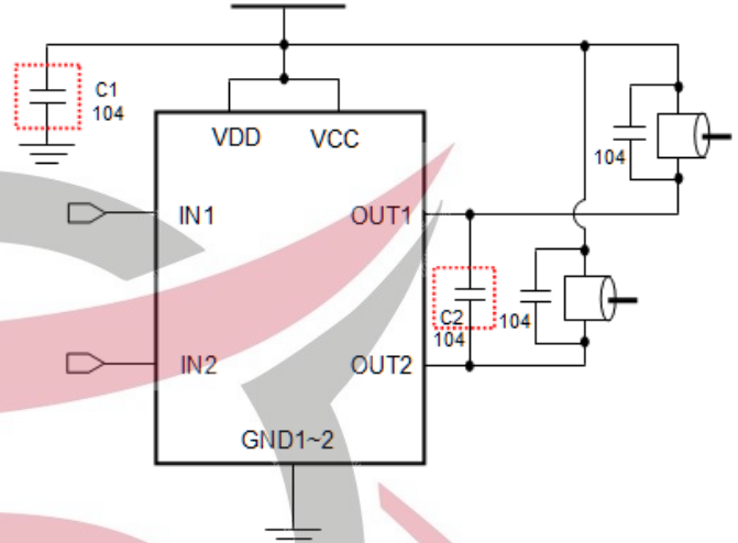
(2) Two Motors Directional Control (Single Power)
